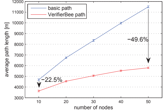
Fig. 13. Average path length wrt the number of nodes. Each point stems from 100 experiments. 95%-confidence intervals are displayed in error bars.
