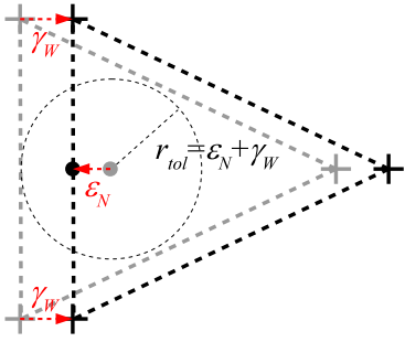
Fig. 4. Error tolerance in the worst case. The visited waypoints (black crosses) are shifted wrt the planned ones (gray crosses). The real node's position (black dot) is shifted wrt the supposed one (gray dot).
