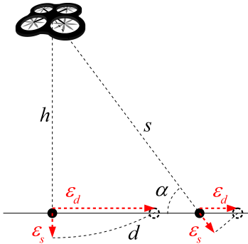
Fig. 5. Ground precision. If the drone is above the ranged node, a small imprecision on the slant distance ( \epsilon_s ) will translate into a huge imprecision on the ground one ( \epsilon_d ).
